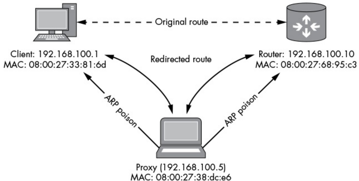
Figure 4-10: ARP poisoning
