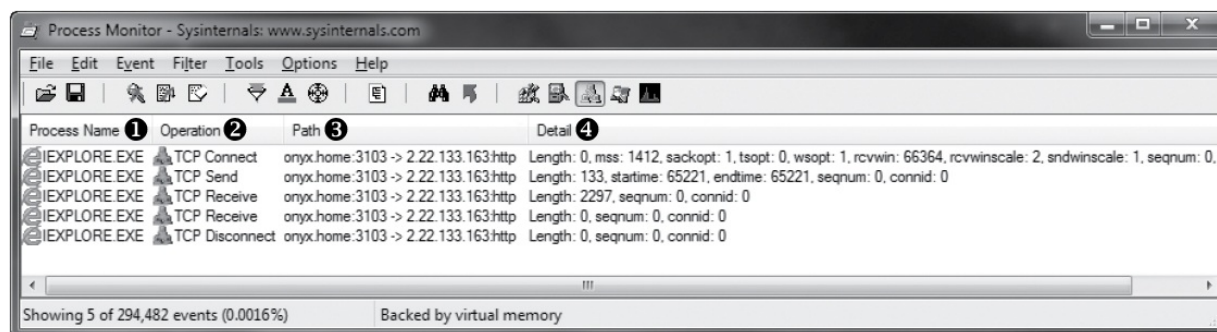
Figure 2-6: A single captured connection
