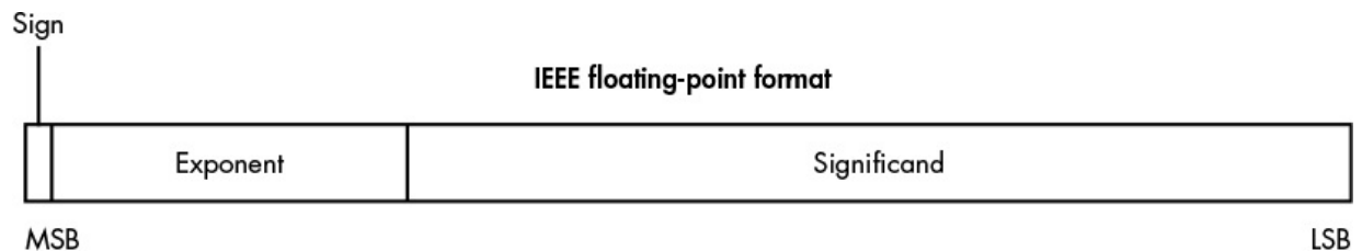
Figure 3-4: Floating-point representation
